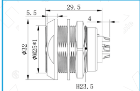
ECG(双螺母安装)
